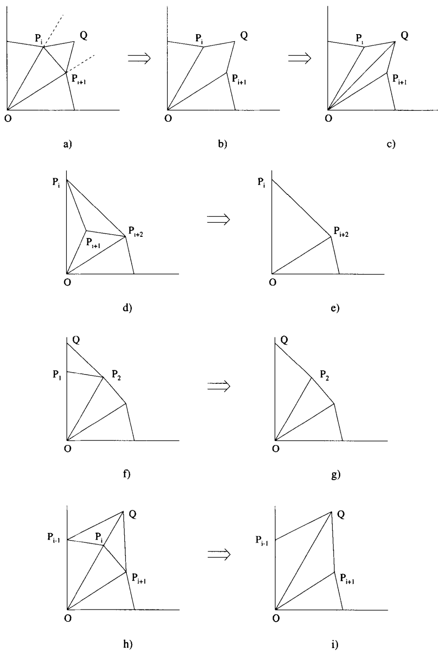
Figure 2. Transformation of a triangulation.
